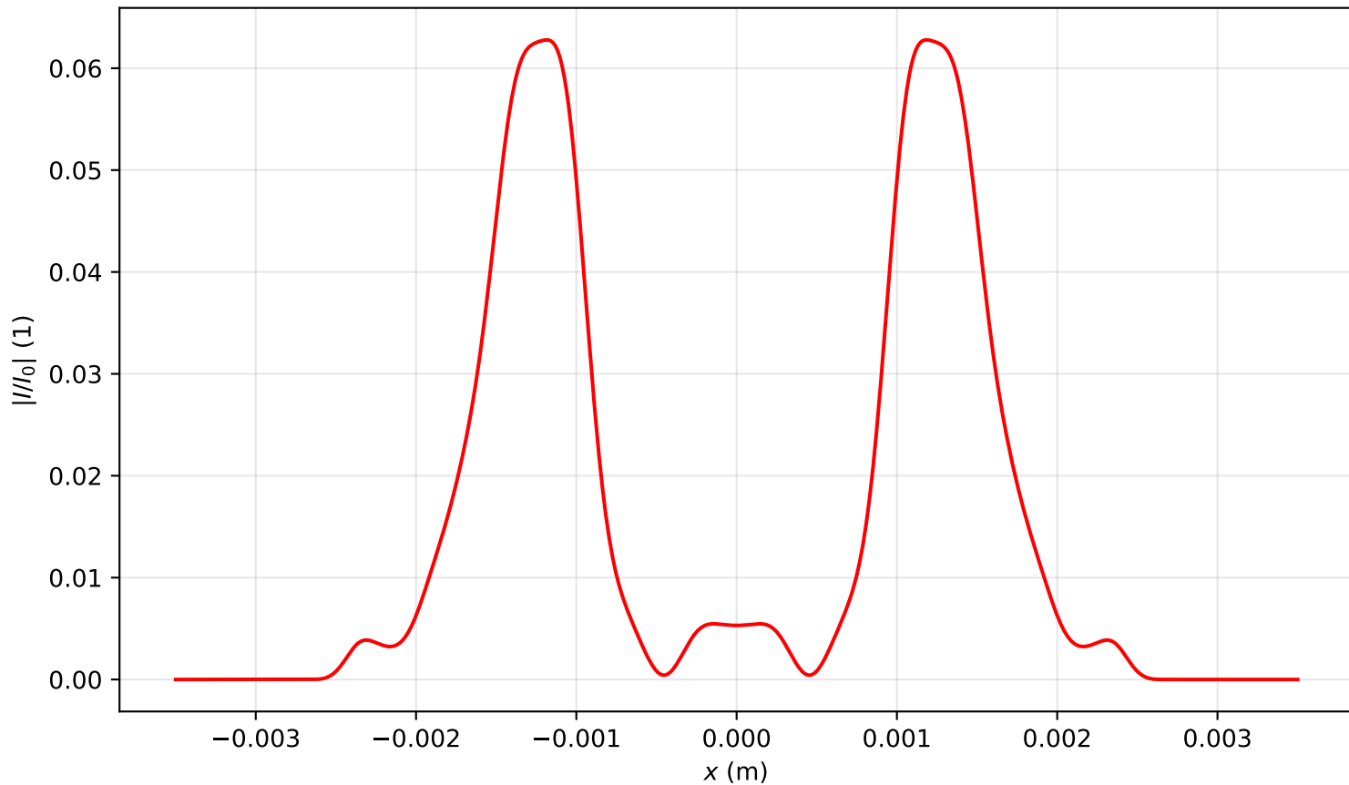
Intensity profile I(x, y = 0, z = 3.821)/I_0 , P_{in}=7.5P_{cr} , artificial time
